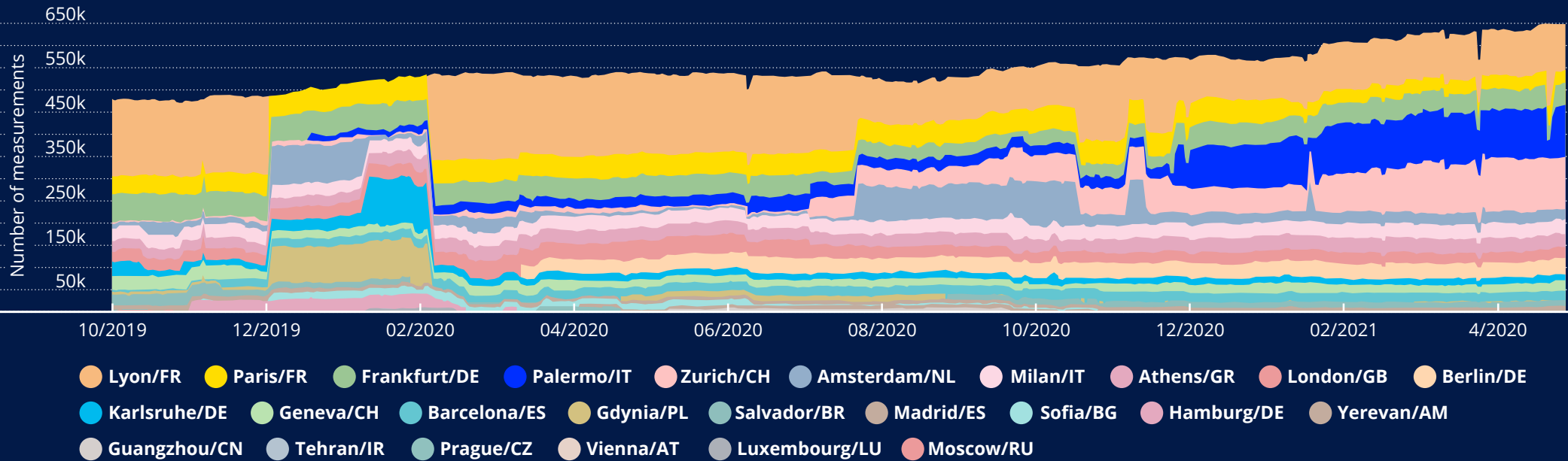
Figure 22: K-root locations reached from within Mediterranean Europe (IPv4)
