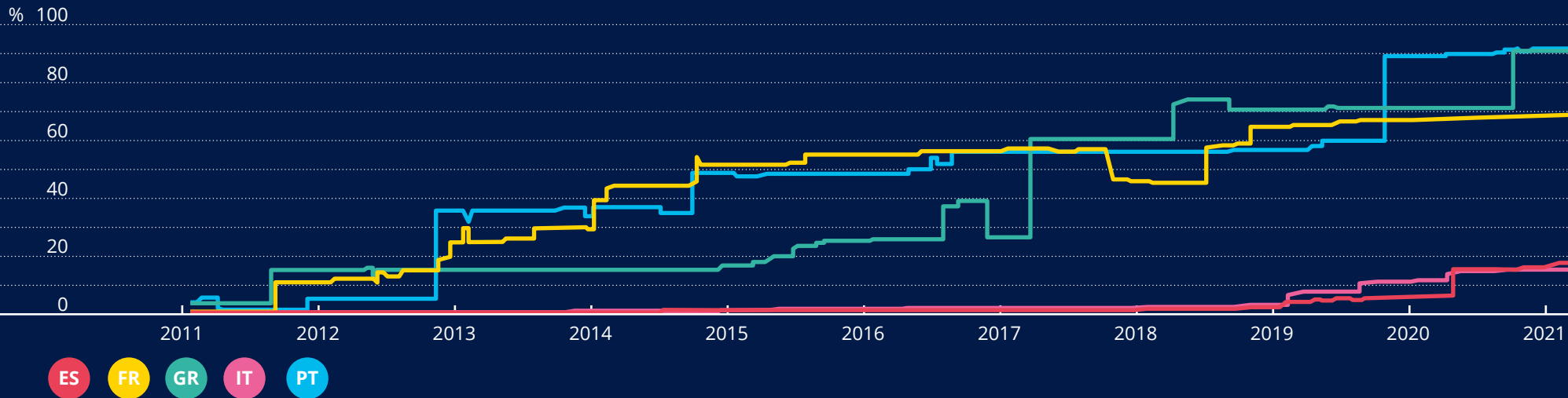
Figure 29: IPv4 address space covered by RPKI
